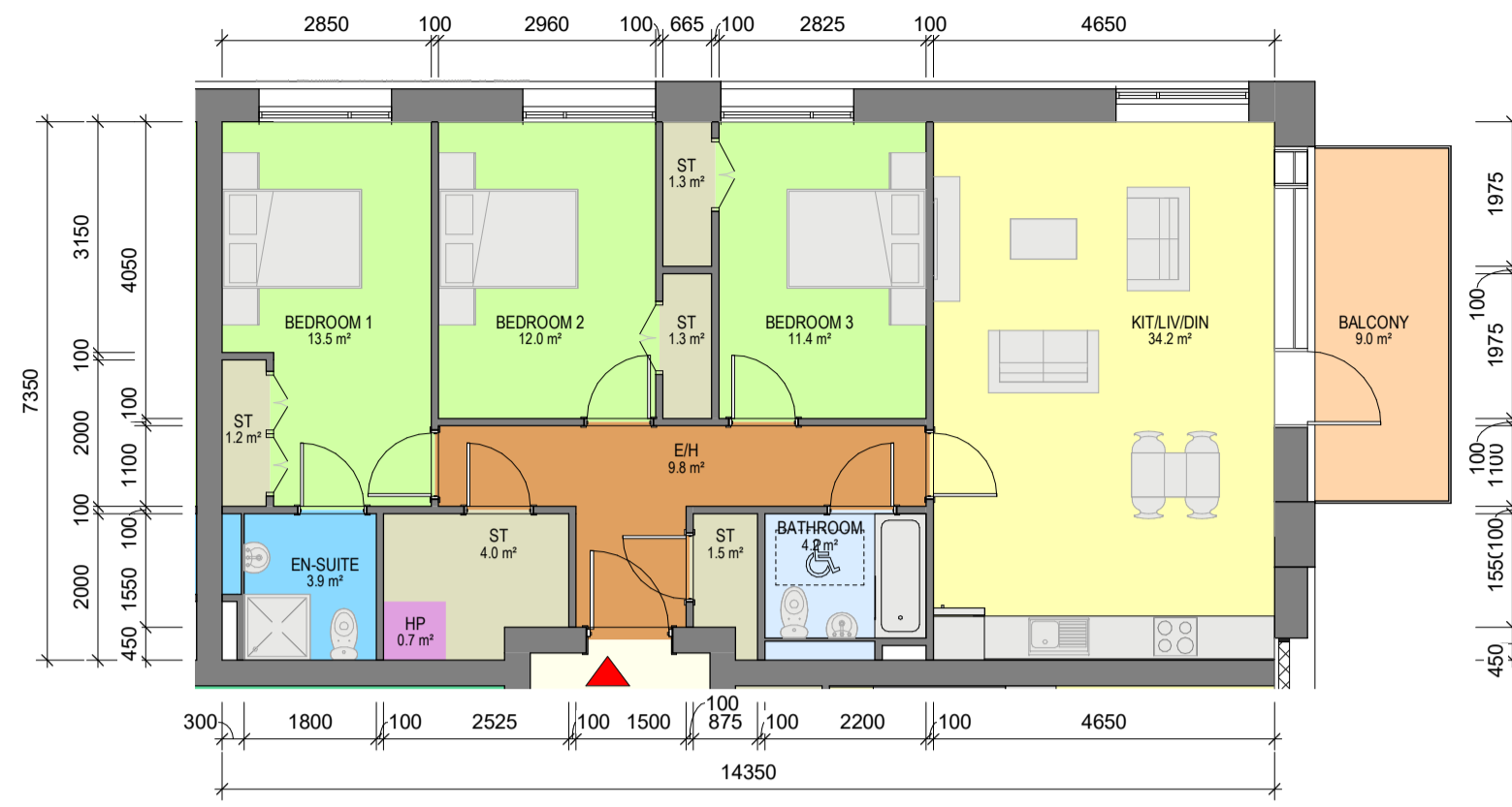
1 Apartment Type 3A 1 : 100
